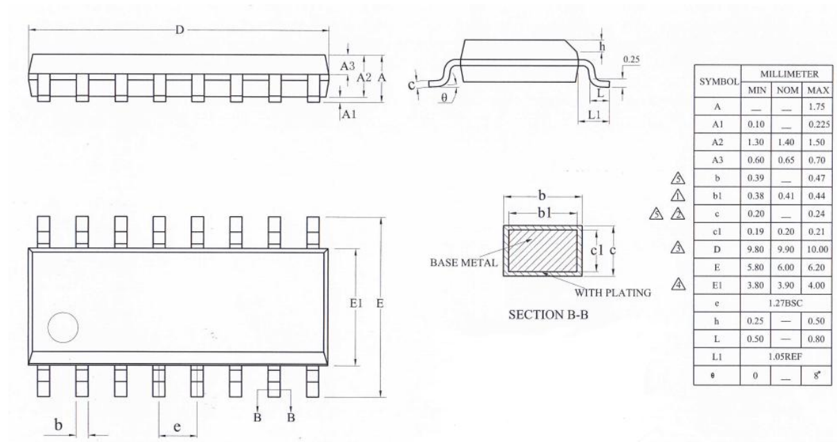
Figure 4-1 AC7069F Package
