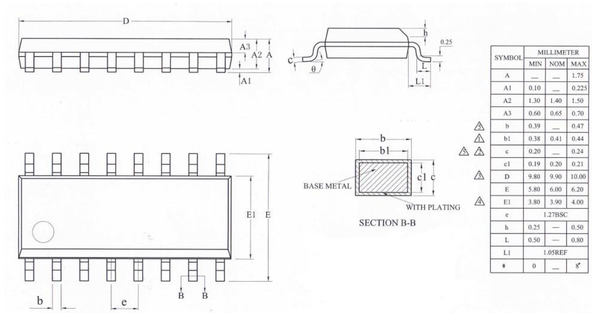
Figure 4-1 AC7069A Package
