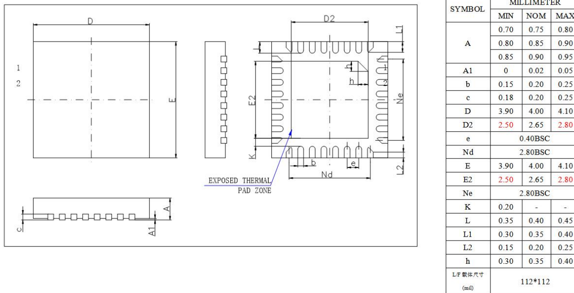
Figure 4-1 AC7066A Package
