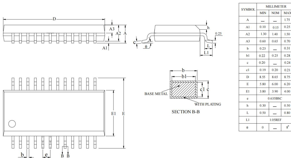
Figure 4-1 AC7065E Package
