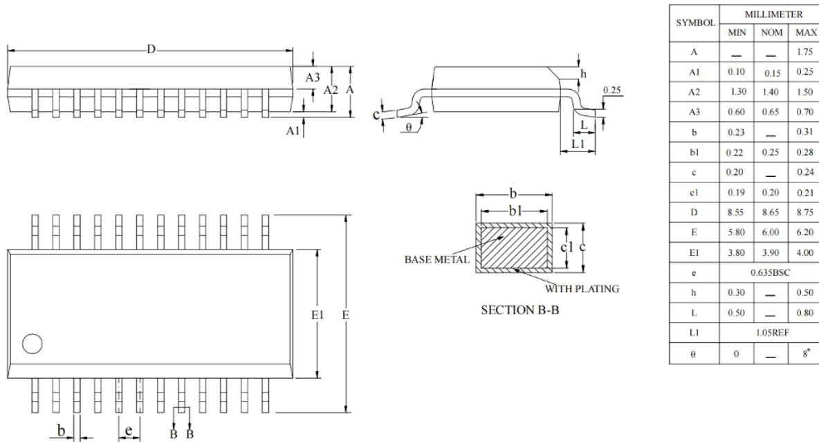
Figure 4-1 AC7065D Package
