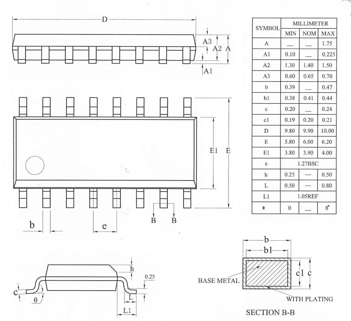
Figure 3-1. AC6969E_SOP16 Package
