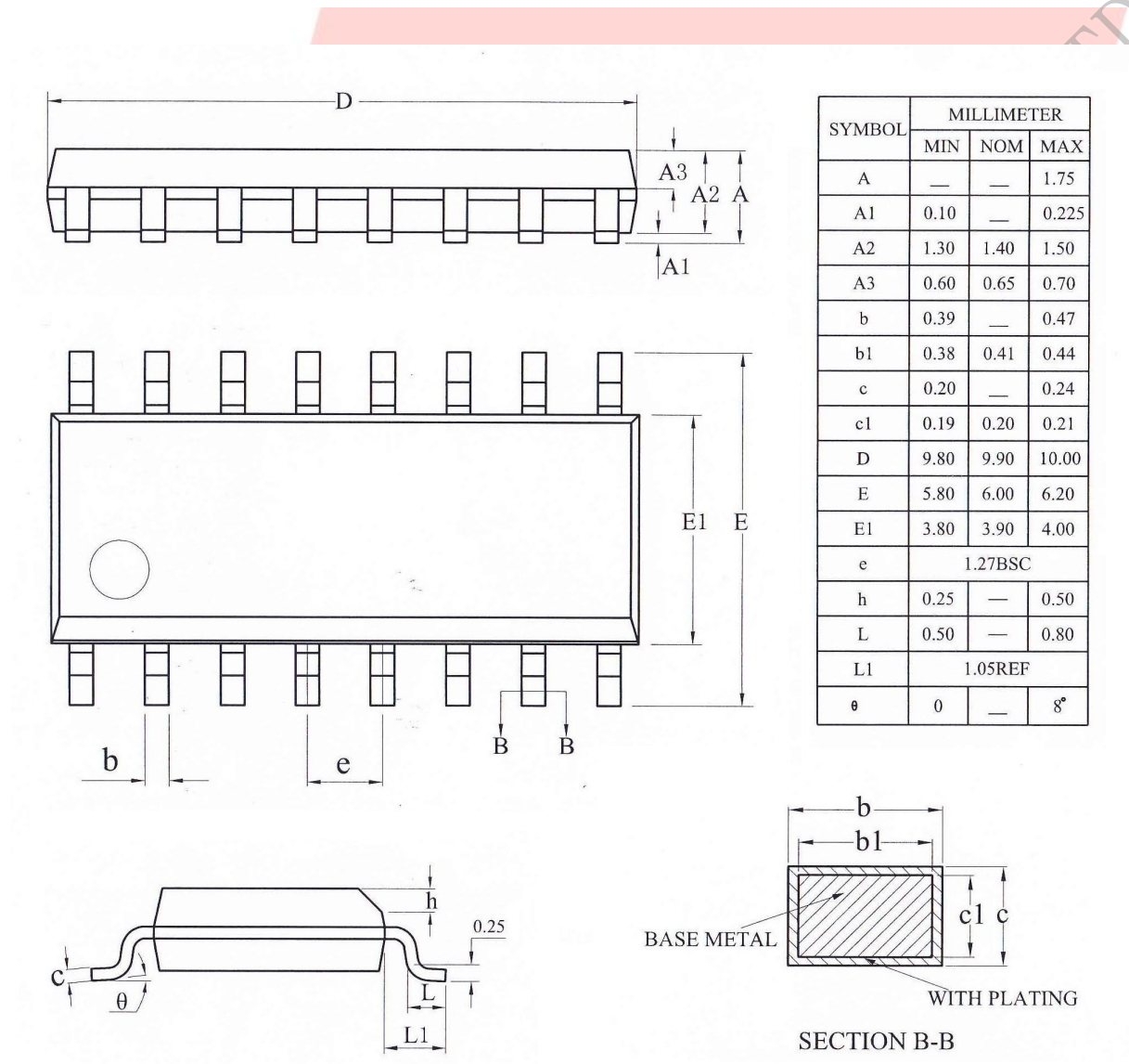
Figure 3-1. AC6969D_SOP16 Package
