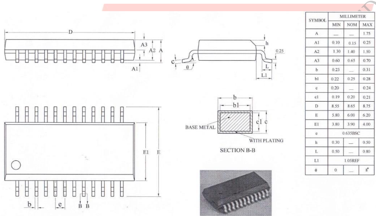
Figure 3-1. AC6965A Package
