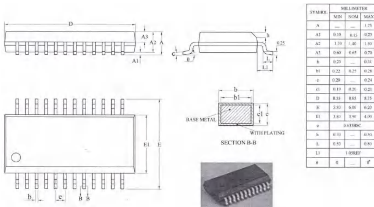
Figure 3-1. AC6965E_QSOP24 Package
