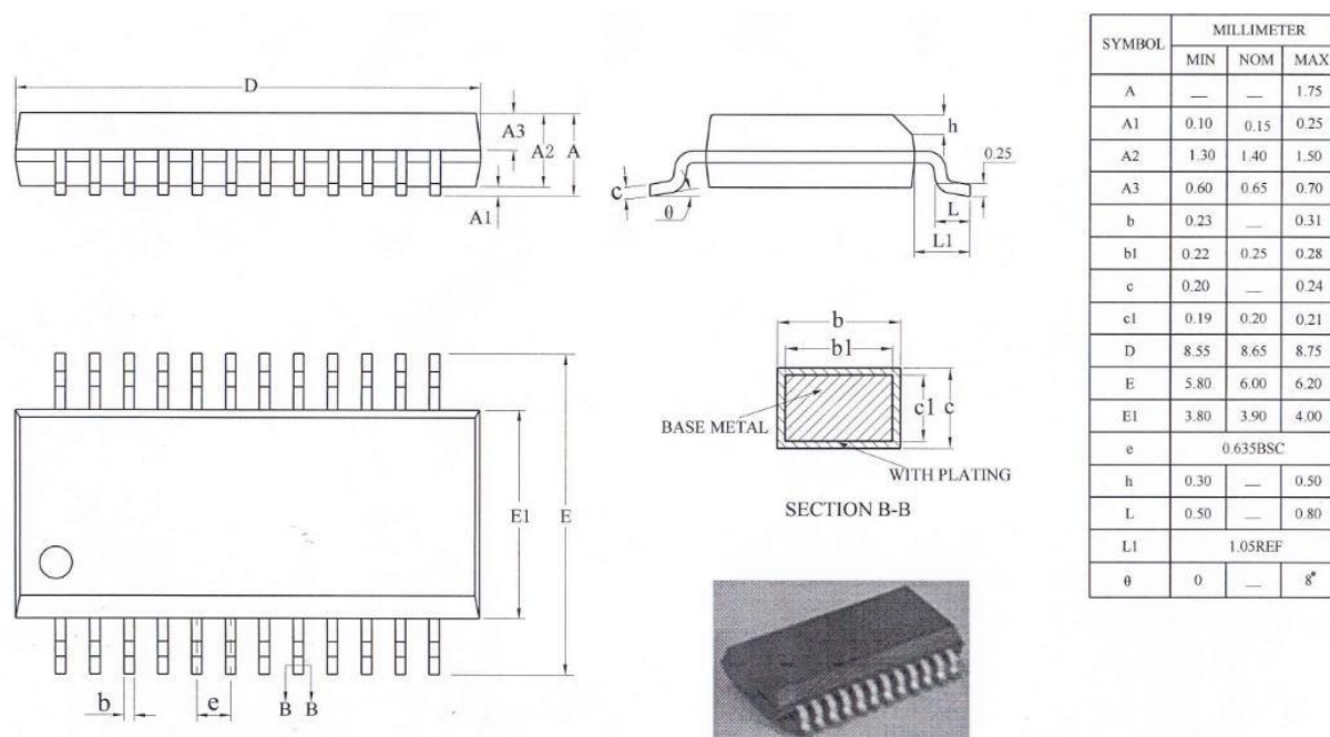
Figure 3-1. AC6965D_QSOP24 Package
