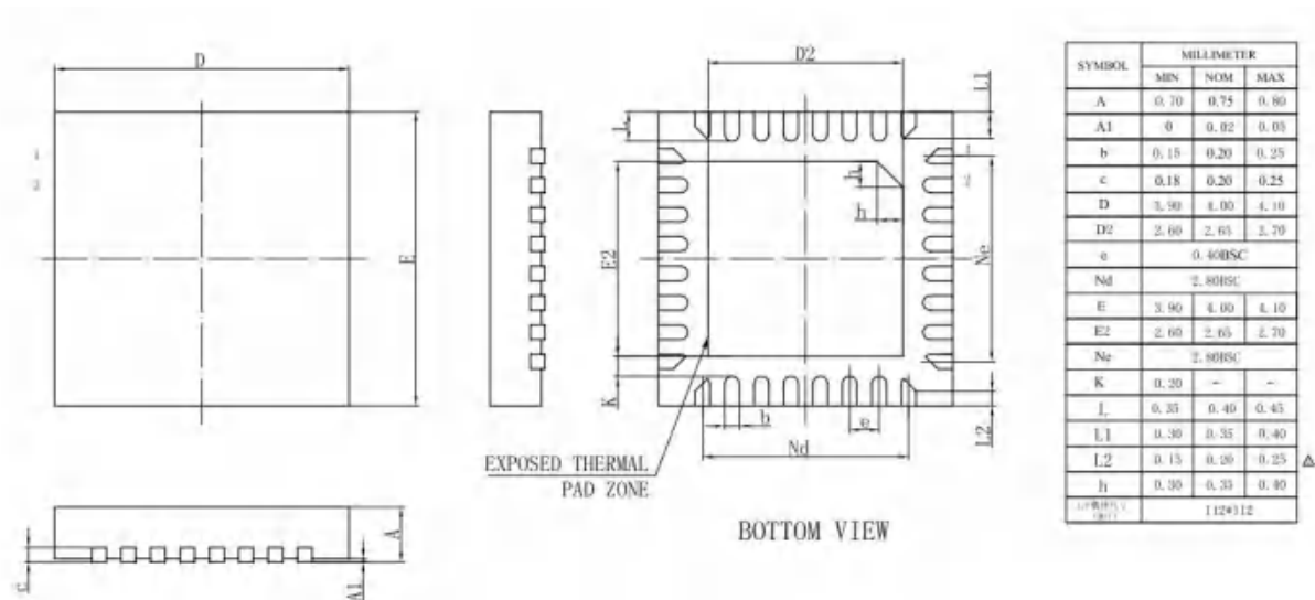
Figure 3-1 AC6956A_QFN32_4x4 Package
