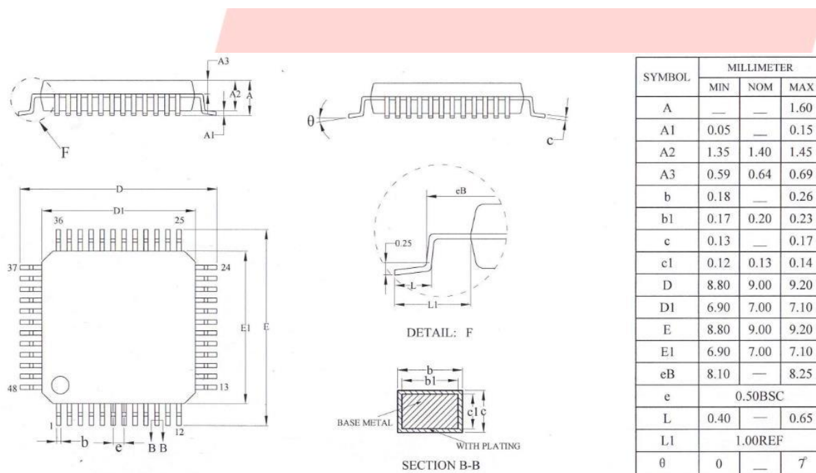
Figure 3-1. AC6951C Package
